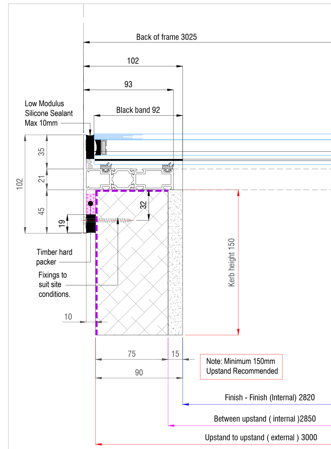
SECTION A-A Scale 1:2 @ A1
