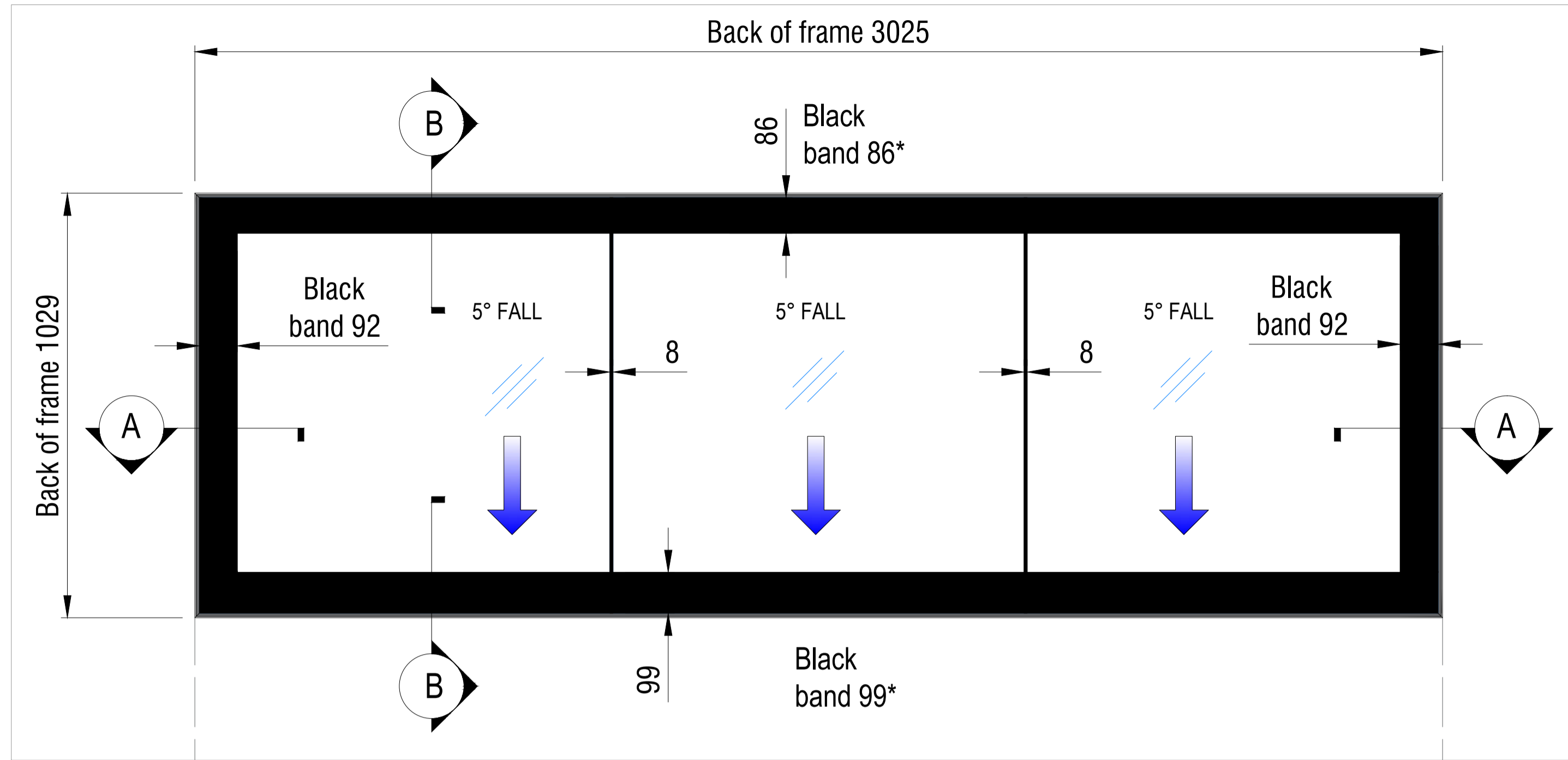
TOP VIEW Scale 1:10 @ A1
